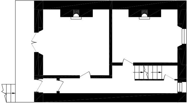
UPPER GROUND FLOOR APPROX. FLOOR AREA 50.1 SQ.M. (539 SQ.FT.)
